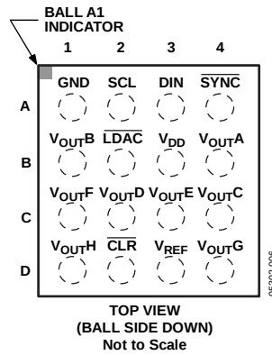
Figure 6. 16-Lead WLCSP
