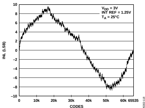
Figure 19. INL AD5668-1
