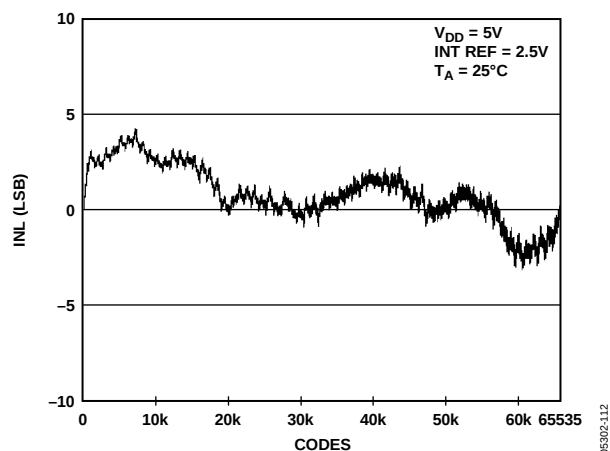
Figure 13. INL AD5668-2/AD5668-3
