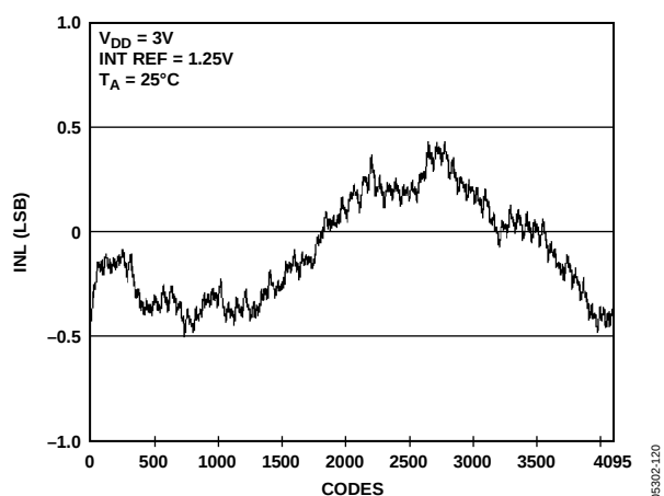
Figure 21. INL AD5628-1
