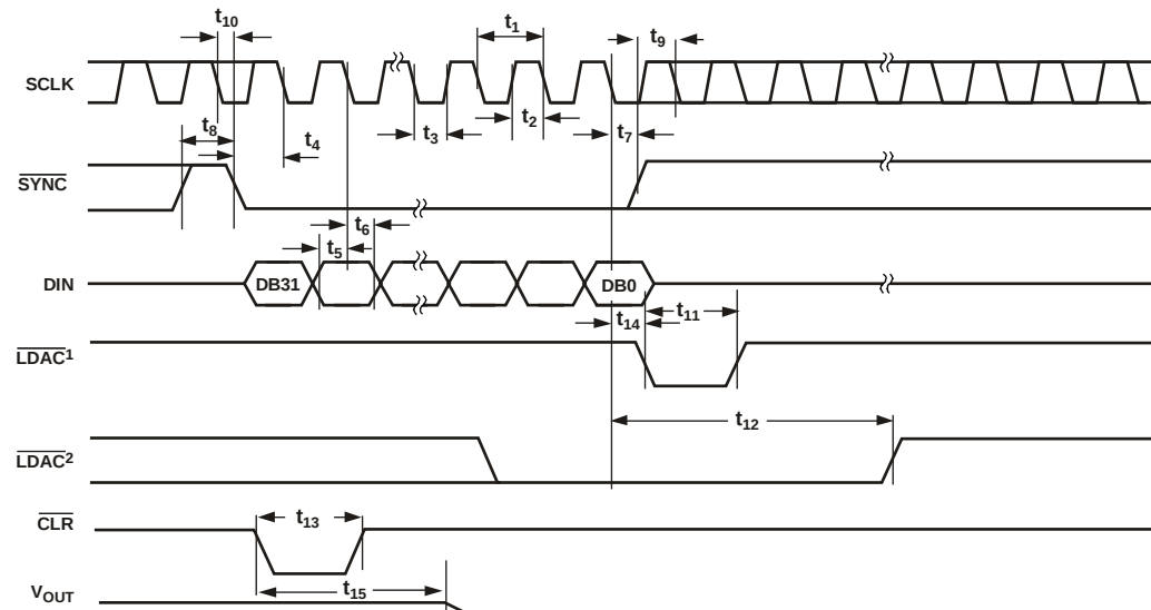
Figure 2. Serial Write Operation
