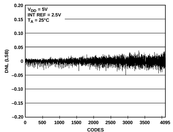
Figure 18. DNL AD5628-2
