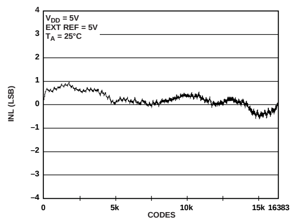
Figure 14. INL AD5648-2
