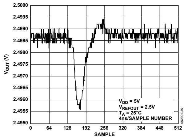
Figure 35. Analog Crosstalk
