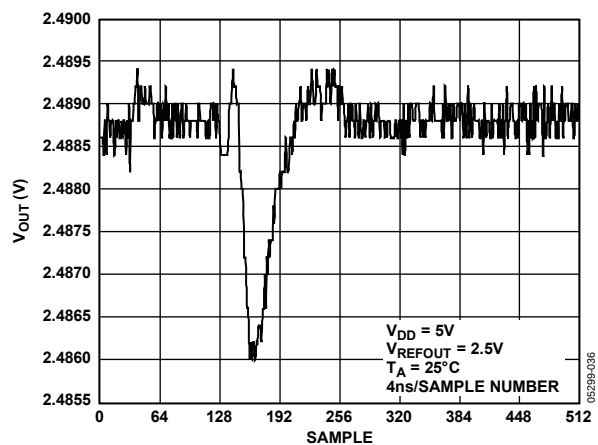
Figure 36. DAC-to-DAC Crosstalk
