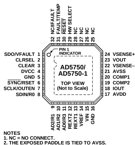
Figure 4. Pin Configuration
