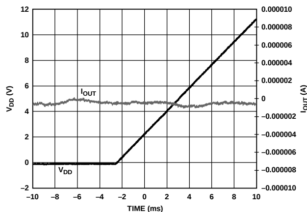
Figure 45. Output Current vs. Time on Power-Up
