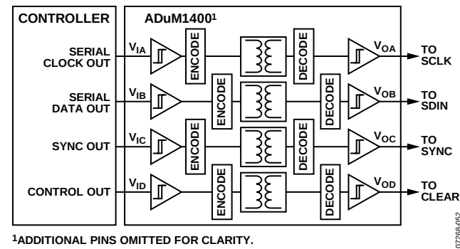
Figure 58. Isolated Interface
