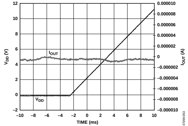
Figure 44. Output Current vs. Time on V_{DD} Power-Up
