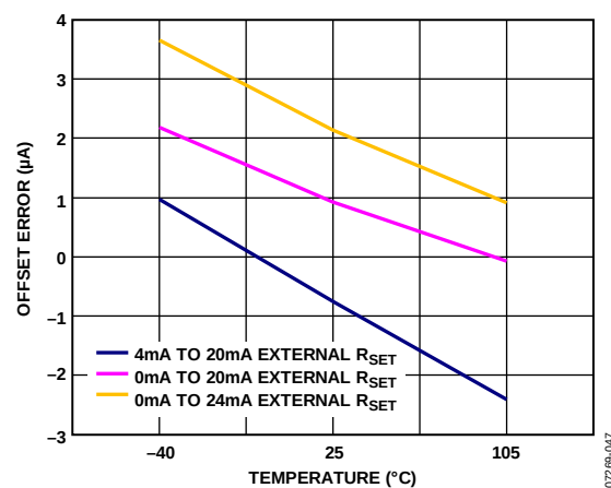
Figure 38. Offset Error vs. Temperature, External R_{SET} Sense Resistor
