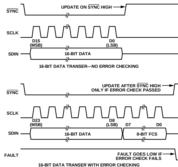
Figure 54. PEC Error Checking Timing
