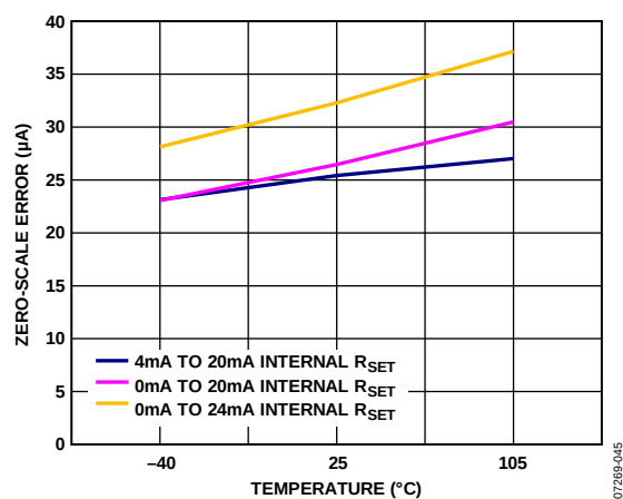
Figure 36. Zero-Scale Error vs. Temperature, Internal R_{SET} Sense Resistor
