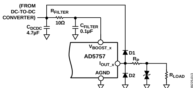
Figure 63. Output Transient Voltage Protection
