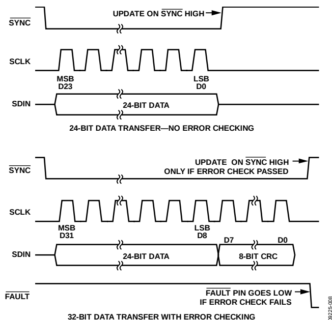
Figure 54. PEC Timing
