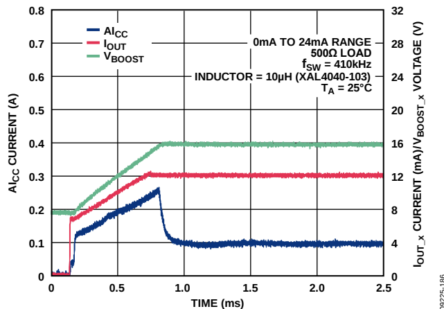
Figure 60. I_{CC} Current vs. Time for 24 mA Step Through 500 \Omega Load with External 51 k \Omega Compensation Resistor
