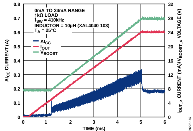
Figure 61. I_{CC} Current vs. Time for 24 mA Step Through 1 k \Omega Load with Slew Rate Control
