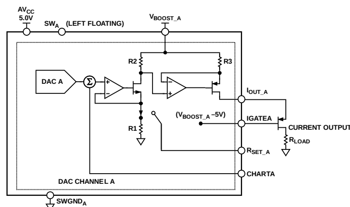
Figure 62. Configuration off a Particular Channel Using IGATE
