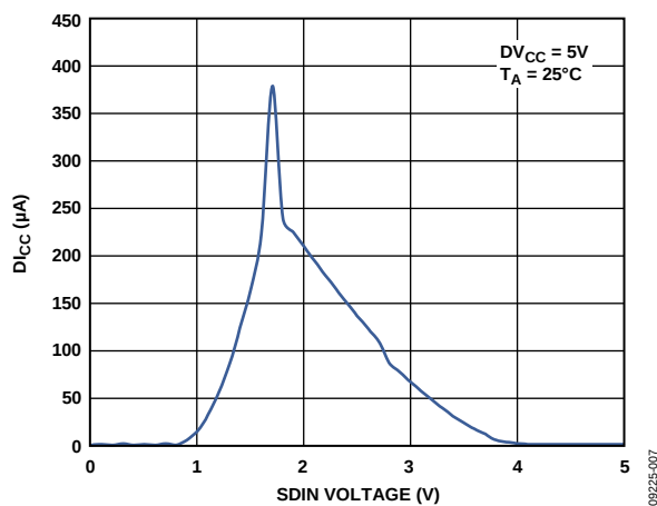
Figure 44. D_{ICC} vs. Logic Input Voltage
