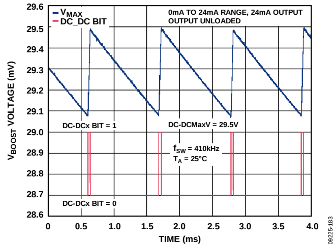
Figure 57. Operation on Reaching V MAX
