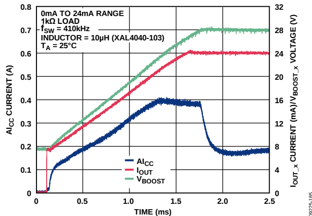
Figure 59. I_{CC} Current vs. Time for 24 mA Step Through 1 k \Omega Load with External 51 k \Omega Compensation Resistor
