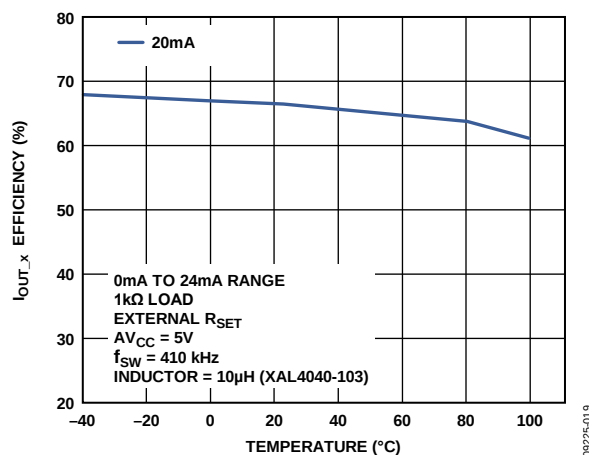
Figure 36. Output Efficiency vs. Temperature (See Figure 56)
