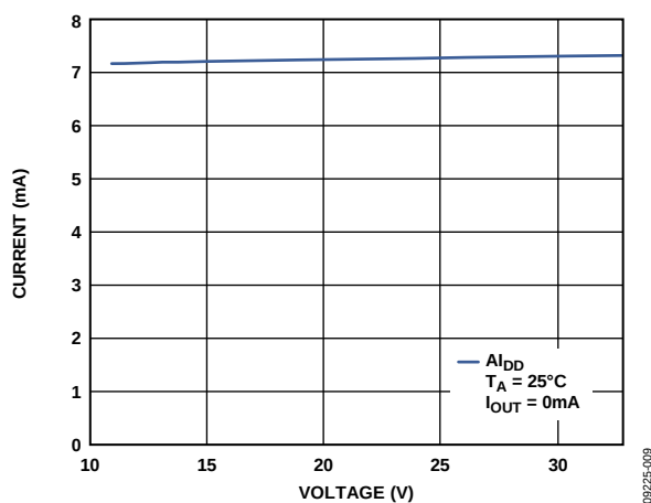
Figure 45. A_{IDD} vs. AV_{DD}
