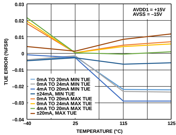
Figure 38. Total Unadjusted Error vs. Temperature, External RSET
