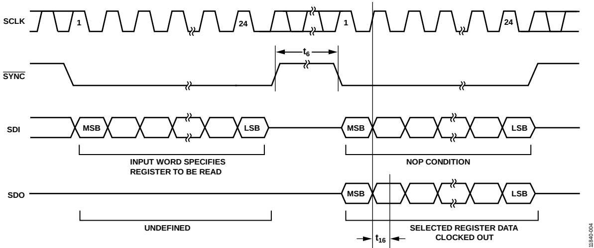
Figure 3. Readback Timing Diagram
