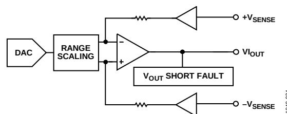
Figure 75. Voltage Output
