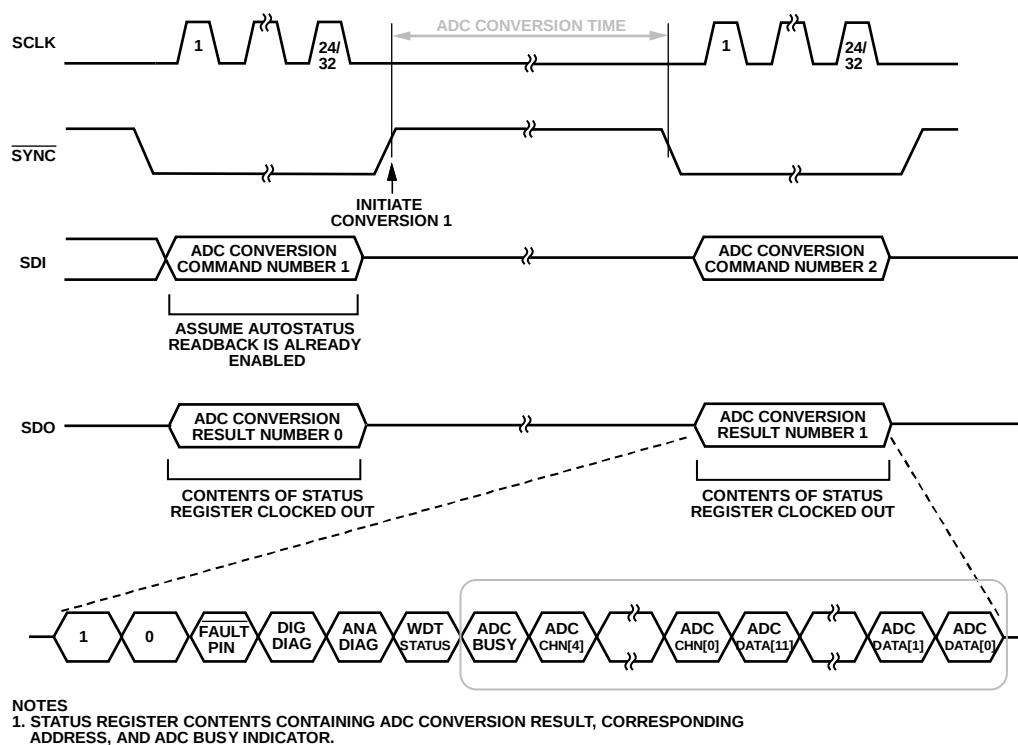
Figure 85. ADC Conversion Timing Example
