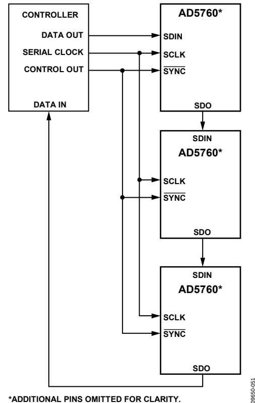
Figure 51. Daisy-Chain Block Diagram
