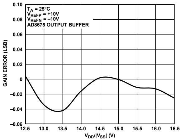
Figure 26. Gain Error vs. Supply Voltage, \pm 10 V Span
