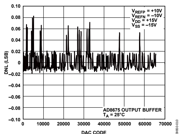
Figure 10. Differential Nonlinearity Error vs. DAC Code, \pm 10 V Span
