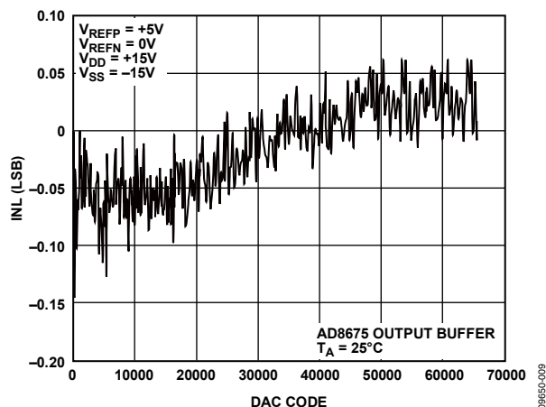
Figure 9. Integral Nonlinearity Error vs. DAC Code, 5 V Span, \times 2 Gain Mode
