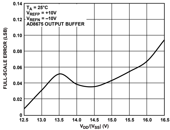
Figure 24. Full-Scale Error vs. Supply Voltage, \pm 10 V Span
