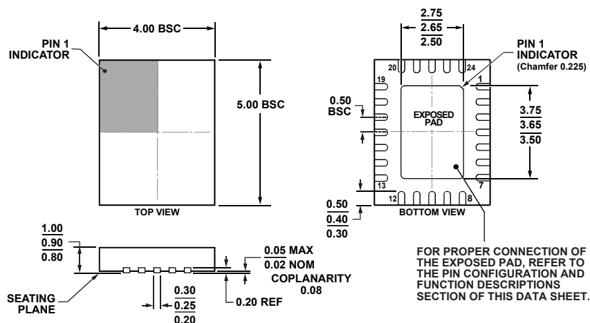
Figure 56. 24-Lead Lead Frame Chip Scale Package [LFCSP_VQ] 4 mm x 5 mm, Very Thin Quad (CP-24-5) Dimensions shown in millimeters
