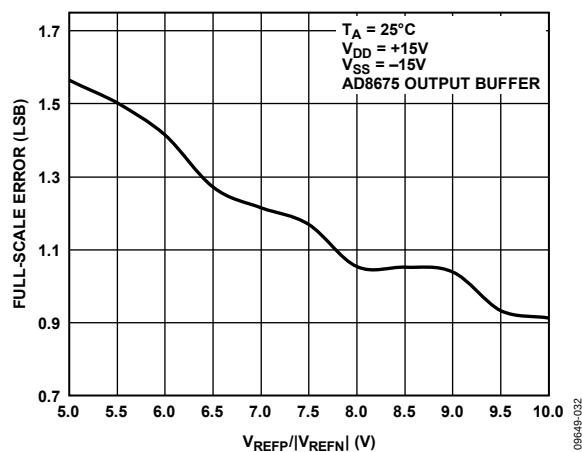
Figure 32. Full-Scale Error vs. Reference Voltage
