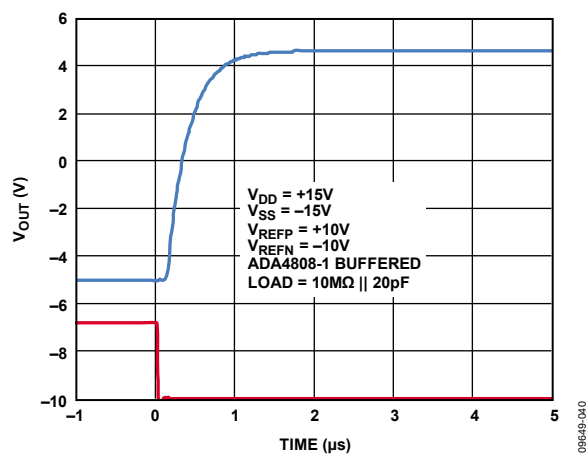
Figure 40. Rising Full-Scale Voltage Step
