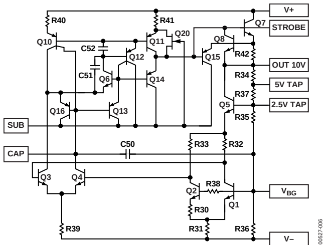
Figure 5. Schematic Diagram
