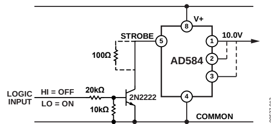
Figure 11. Use of the Strobe Terminal
