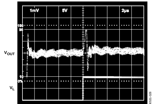
Figure 28. Load Crosstalk
