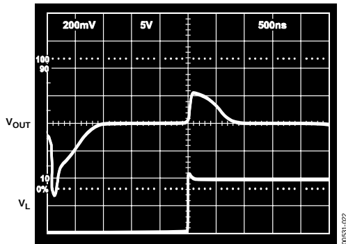
Figure 22. Large-Scale Transient Response
