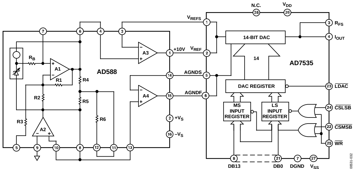
Figure 32. AD588/AD7535 Connections
