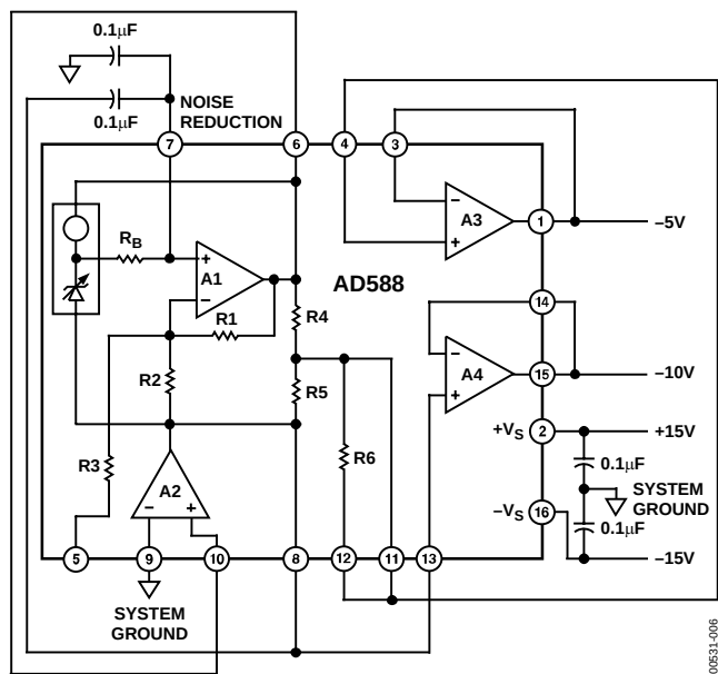
Figure 6. -10 V Output
