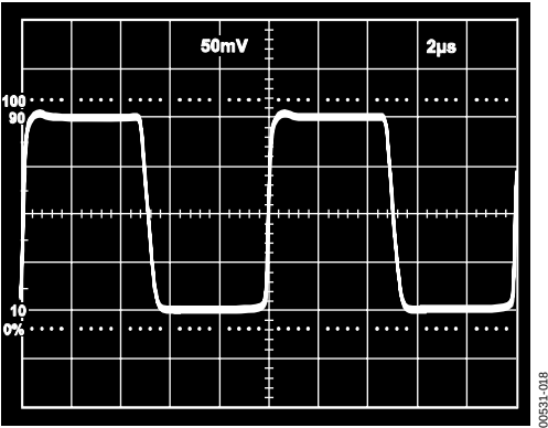
Figure 17. Unity-Gain Follower Pulse Response (Large Signal)
