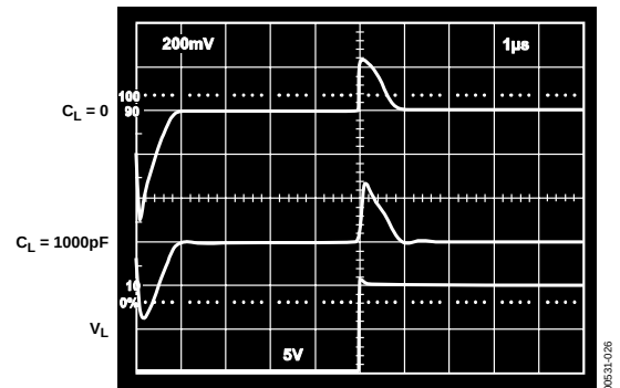
Figure 26. Output Response with Capacitive Load
