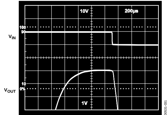
Figure 30. Output Amplifier Step Response Using Figure 31 Compensation
