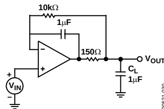
Figure 31. Compensation for Capacitive Loads
