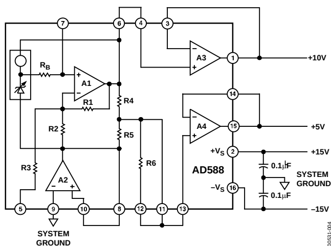
Figure 4. +10 V Output
