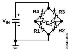
Figure 38. Bridge Transducer Excitation—Unipolar Drive
