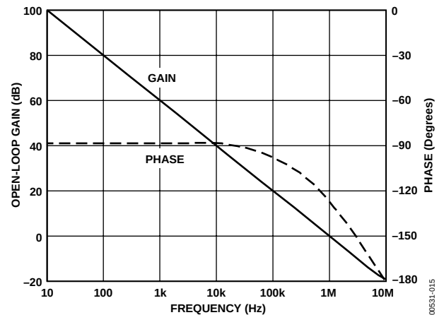
Figure 15. Open-Loop Frequency Response (A3, A4)
