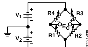
Figure 39. Bridge Transducer Excitation—Bipolar Drive
