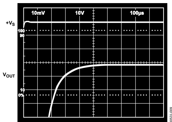
Figure 9. Electrical Turn-On
