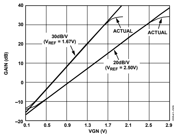
Figure 5. Gain vs. VGN for Different Gain Scalings
