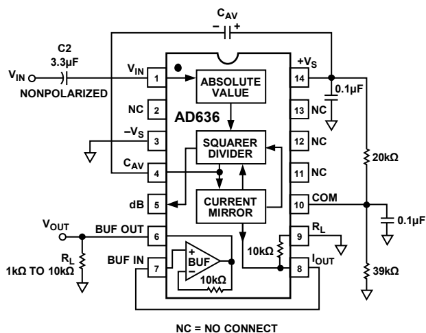
Figure 6. Single-Supply Connection
