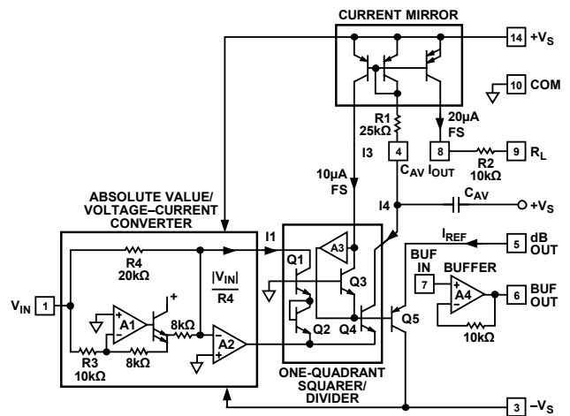
Figure 12. Simplified Schematic
