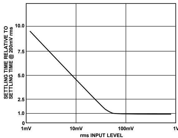
Figure 9. Settling Time vs. Input Level
