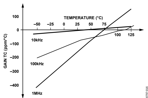
Figure 15. Gain TC vs. Temperature
