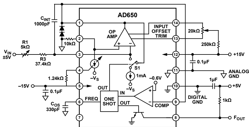
Figure 11. Connections for \pm 5 V Bipolar V/F with 0 kHz to 100 kHz TTL Output Rev. D | Page 10 of 20
