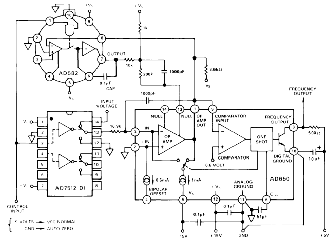
Figure 13. Autozero Circuit
