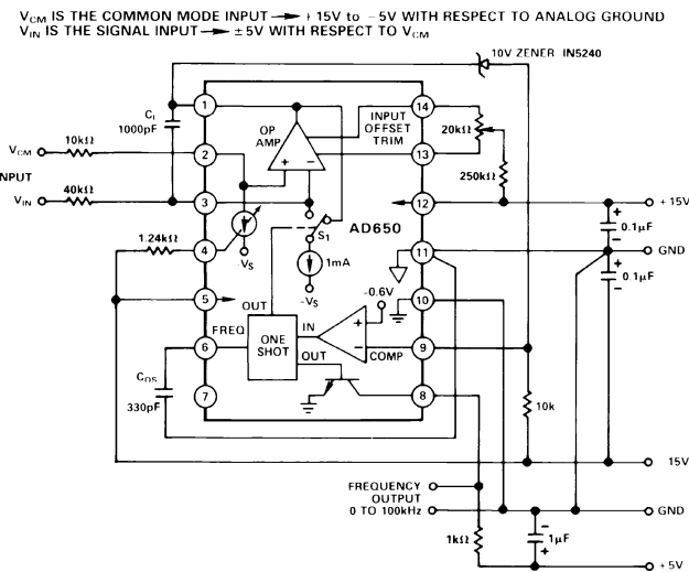
Figure 12. Differential Input
