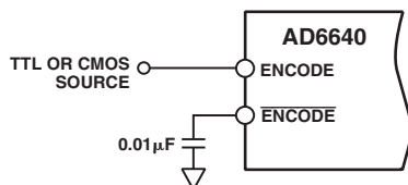
Figure 7. Single-Ended TTL/CMOS ENCODE
