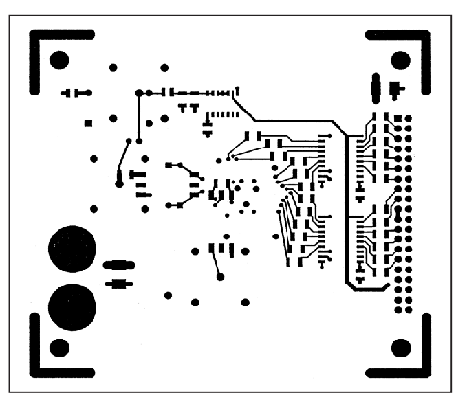
Figure 22. AD6640ST/PCB Bottom Side Copper (Positive)
