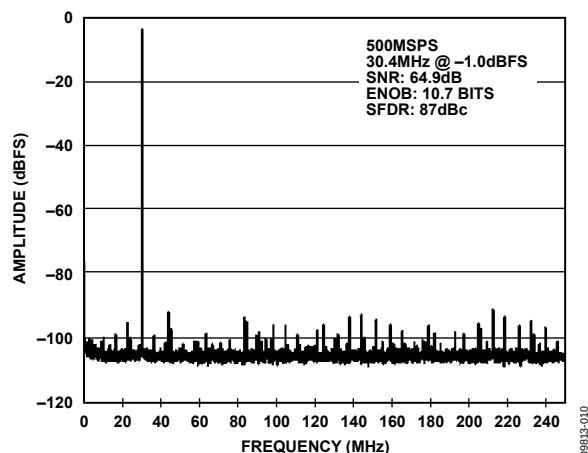
Figure 10. 16k Point Single-Tone FFT; 500 MSPS, 30.4 MHz
