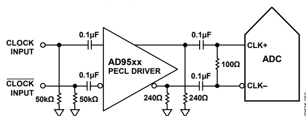
Figure 34. Differential PECL Sample Clock (Up to 625 MHz)
