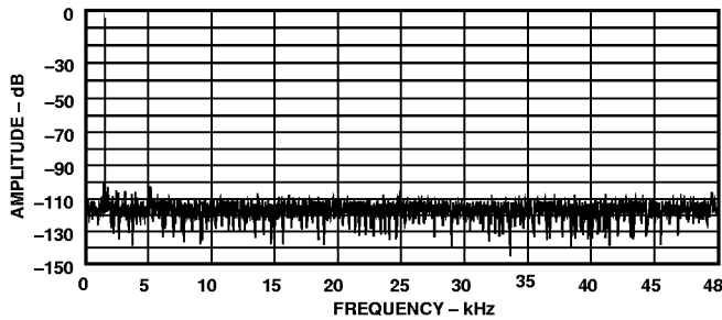
Figure 16. IMD Plot for f_{IN} = 1008 \text{ Hz (fa)} , 1055 \text{ Hz (fb)} at 96 kSPS
