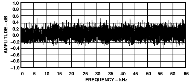
Figure 19. DNL Plot at V_{REF} = 10 \text{ V} , T_A = +25^\circ \text{C} , f_S = 100 kSPS
