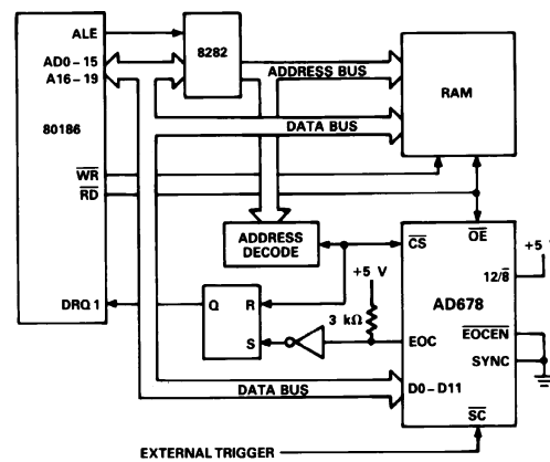
Figure 15. AD678 to 80186 DMA Interface
