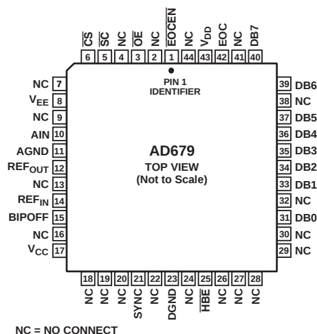
JLCC Package
