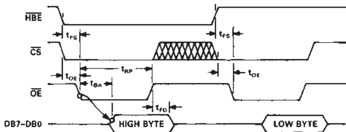
Figure 2. Output Timing
