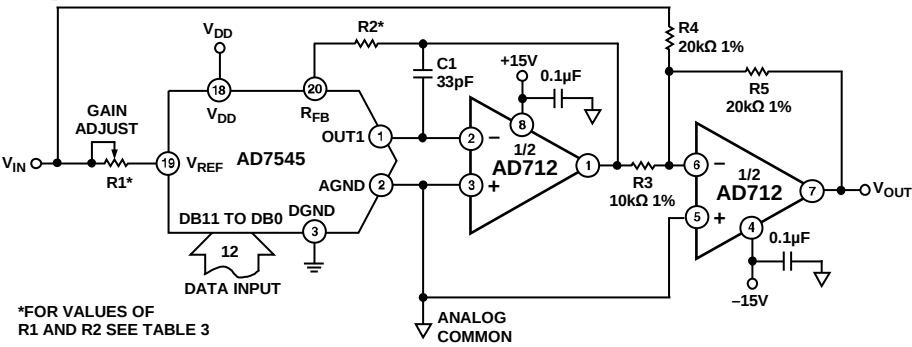
Figure 40. Bipolar Operation
