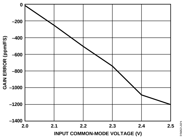
Figure 49. Gain Error vs. Input Common-Mode Voltage, Wideband 0.433 × ODR Filter
