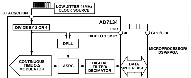
Figure 76. ASRC Slave Mode Functional Diagram
