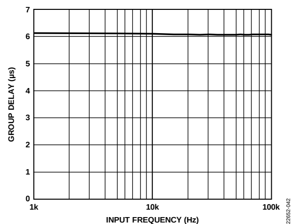
Figure 56. Group Delay vs. Input Frequency, Sinc3 Filter ODR = 1250 kSPS
