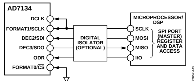
Figure 122. Signal Connection Diagram of Minimum I/O Configuration
