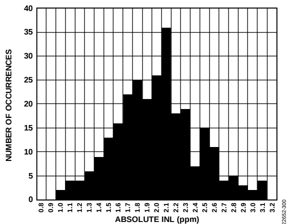
Figure 42. INL Distribution
