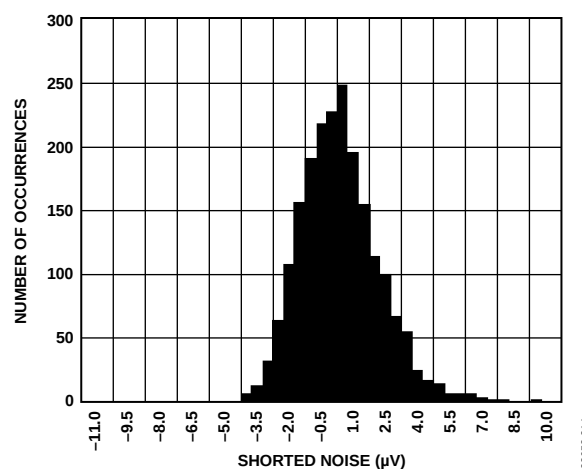
Figure 28. Shorted Noise, Sinc3 Filter
