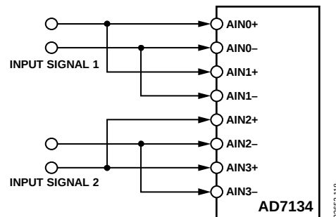
Figure 94. 2:1 Channel Averaging
