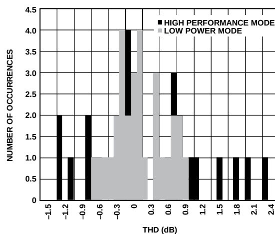
Figure 21. THD Histogram
