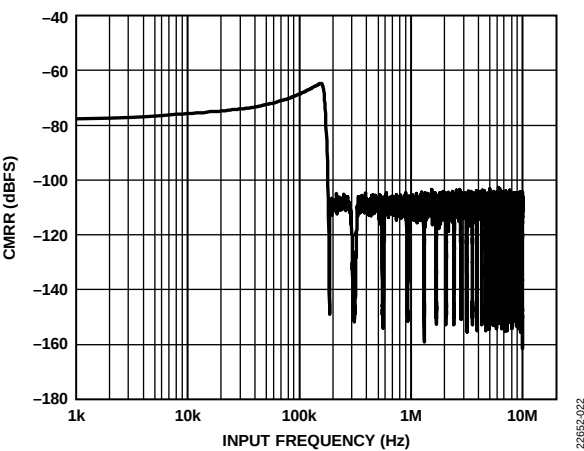
Figure 53. CMRR vs. Input Frequency, Wideband 0.433 × ODR Filter
