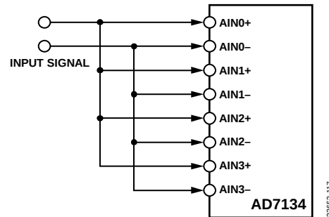
Figure 93. 4:1 Channel Averaging
