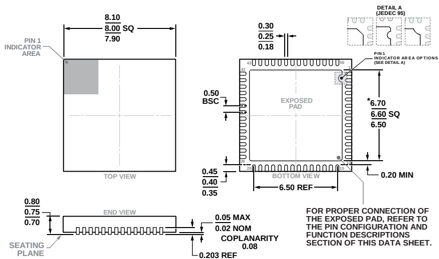
Figure 127. 56-Lead Lead Frame Chip Scale Package [LFCSP] 8 mm × 8 mm Body and 0.75 mm Package Height (CP-56-9)
