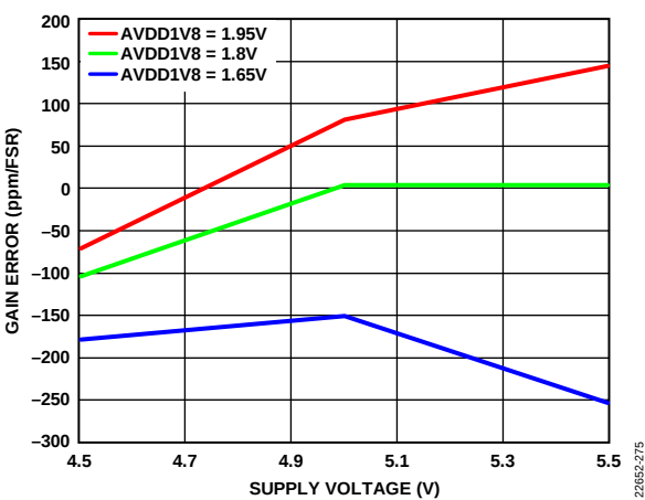
Figure 51. Gain Error vs. Supply Voltage
