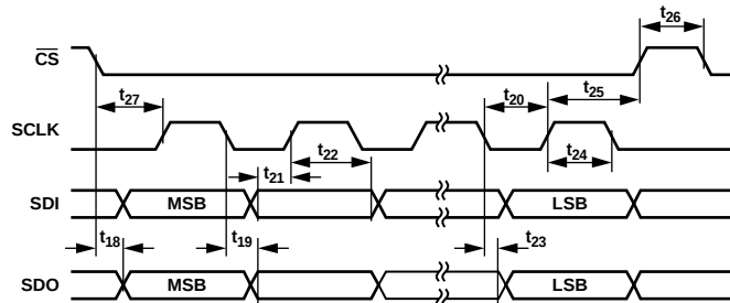
Figure 4. SPI Interface Timing Diagram
