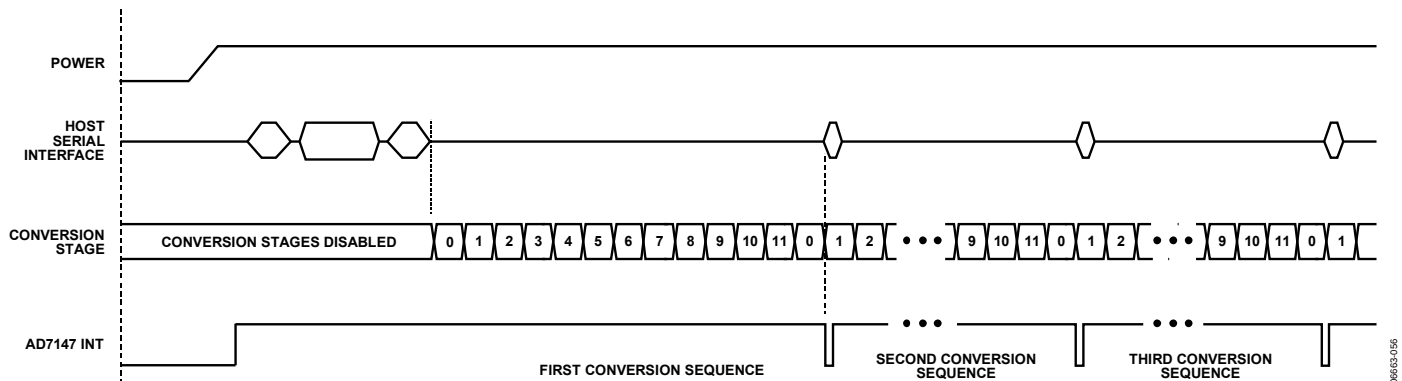
Figure 59. Recommended Start-Up Sequence
