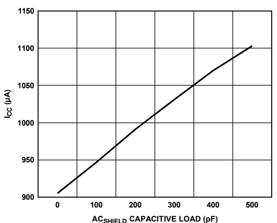
Figure 12. Supply Current vs. Capacitive Load on AC_{SHIELD}
