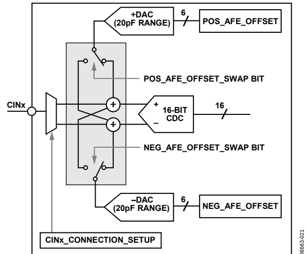
Figure 24. Analog Front-End Offset Control
