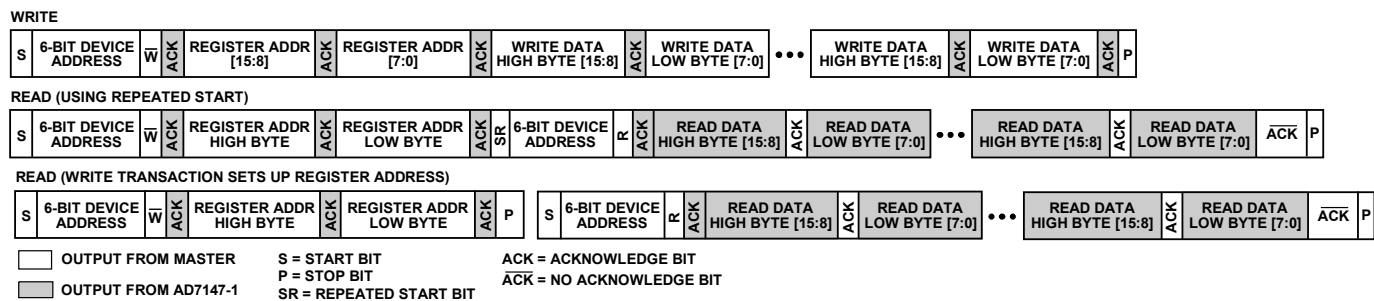
Figure 55. Example of Sequential I²C Write and Readback Operations
