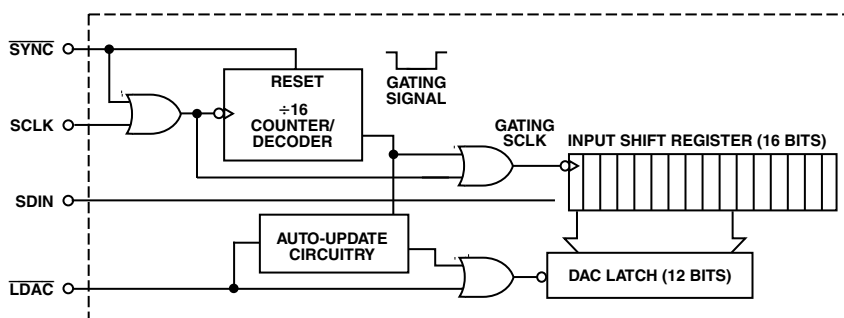
Figure 2. Simplified Loading Structure
