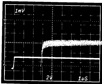
Positive-Going Settling Time (V DD = +15V, V SS = -15V)
