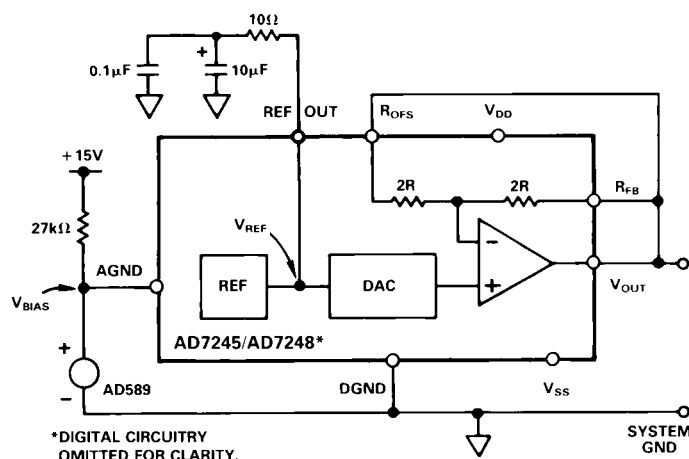
Figure 9. AGND Bias Current
