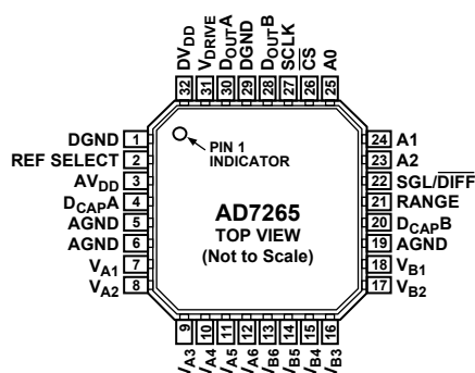
Figure 2. 32-Lead CP-32-2
