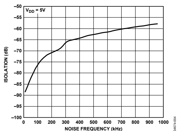
Figure 5. Channel-to-Channel Isolation
