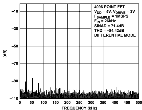
Figure 7. FFT
