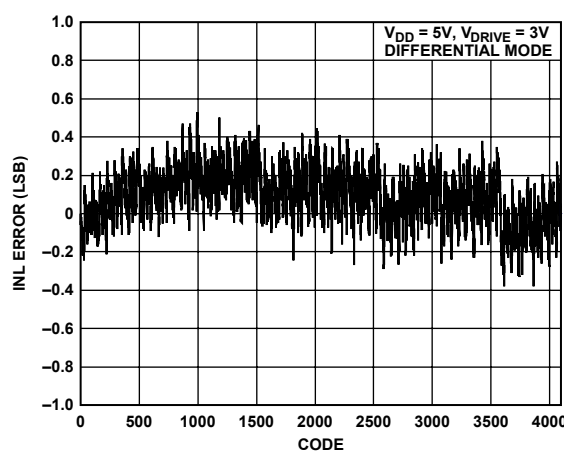
Figure 9. Typical INL
