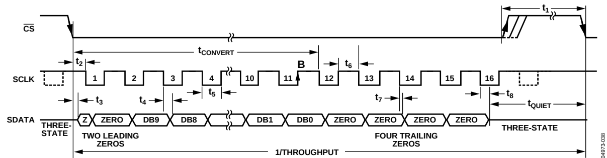
Figure 38. AD7273 Serial Interface Timing Diagram
