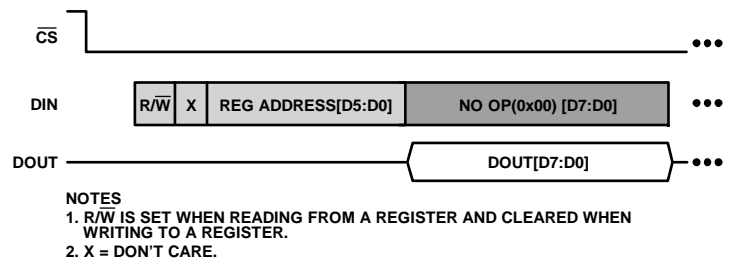
Figure 53. Accessing an 8-Bit Register
