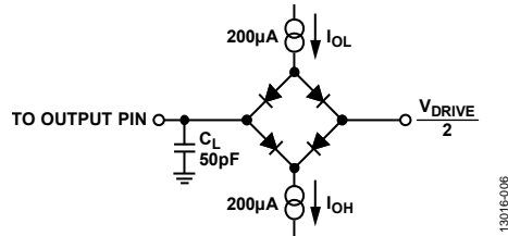
Figure 6. Load Circuit for Digital Output (DOUT) Timing Specifications
