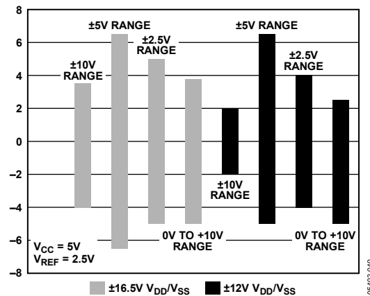
Figure 43. Pseudo Differential Input Range with V_{CC} = 5 V
