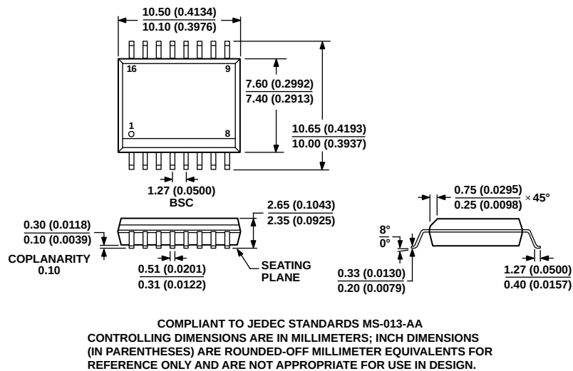
Figure 37. 16-Lead Standard Small Outline Package [SOIC_W] Wide Body (RW-16) Dimensions shown in millimeters and (inches)
