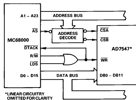
Figure 11. AD7547-MC68000 Interface
