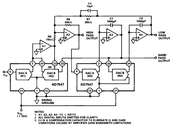
Figure 6. Programmable State Variable Filter
