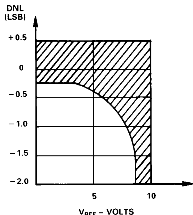
Figure 9. Differential Nonlinearity vs. Reference Voltage for Circuit of Figure 8. V_{DD}=15V . Shaded Area Shows Range of Values of Differential Nonlinearity that Typically Occur for L, C and U Grades
