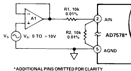
Figure 13. Unipolar 0 to +10V Operation
