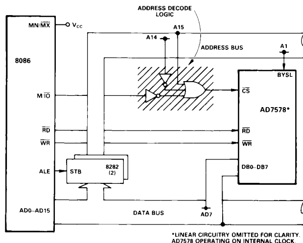
Figure 22. AD7578 – 8086 Interface
