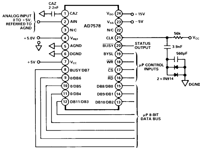
Figure 5. AD7578 Operational Diagram
