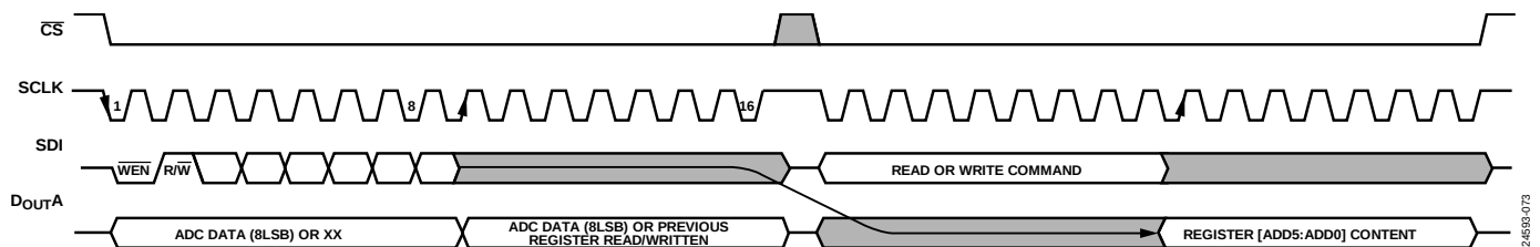
Figure 109. Serial Interface Read Command, First Frame Provides the Address, Second Frame Provides the Register Content
