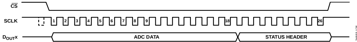
Figure 108. Serial Interface, ADC Mode, Status On
