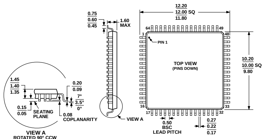
Figure 124. 64-Lead Low Profile Quad Flat Package [LQFP] (ST-64-2)
