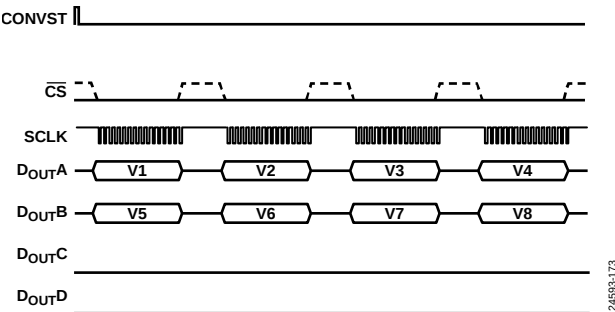
Figure 103. Serial Interface ADC Reading, Two DOUTX Lines
