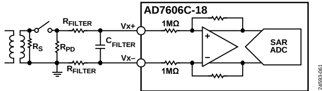
Figure 94. Analog Front End with R_{PD}
