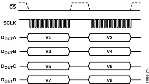
Figure 104. Serial Interface ADC Reading, Four DOUTX Lines
