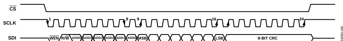
Figure 113. Writing Registers Through the SPI with CRC Enabled
