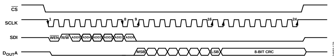
Figure 112. Reading Registers Through the SPI with CRC Enabled
