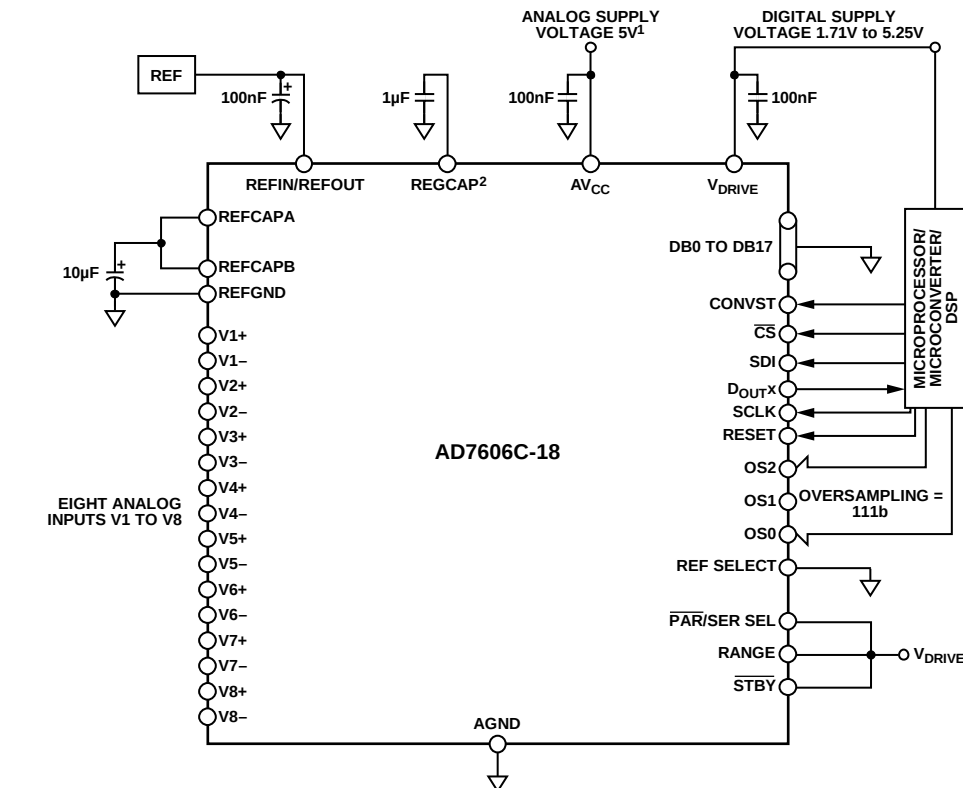
Figure 120. Typical Connection Diagram, Software Mode
