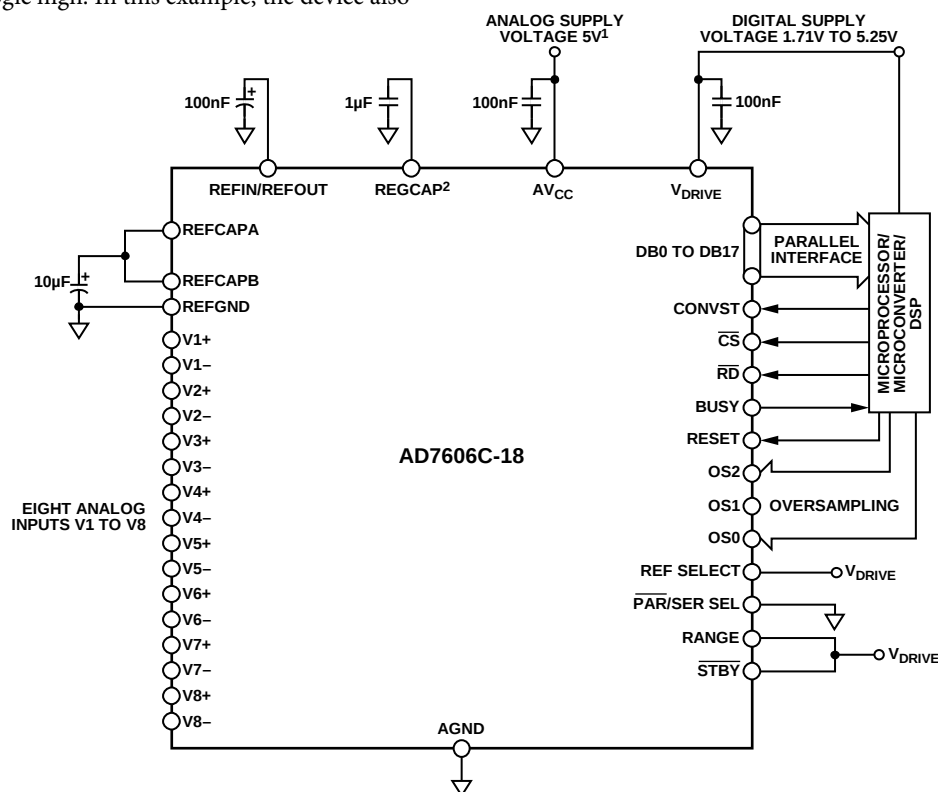
Figure 119. Typical Connection Diagram, Hardware Mode
