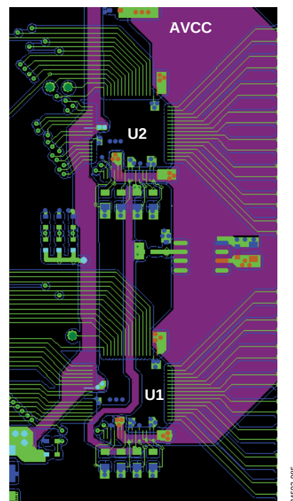
Figure 123. Layout for Multiple AD7606C-18 Devices—Top Layer and Supply Plane Layer
