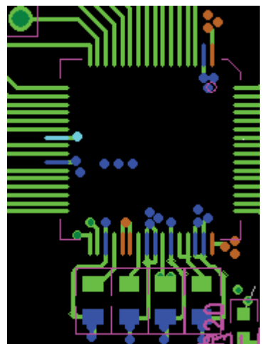
Figure 121. Top Layer Decoupling REFIN/REFOUT, REFCAPA, REFCAPB, and REGCAP Pins
