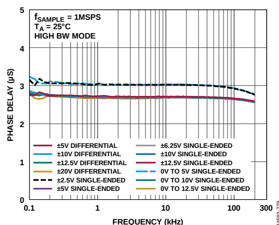
Figure 80. Analog Antialiasing Filter Phase Response, High Bandwidth Mode
