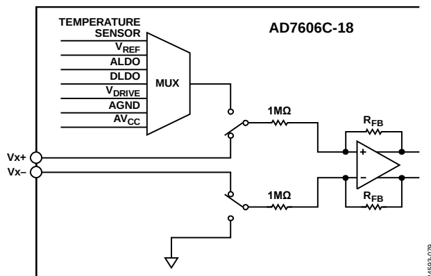
Figure 117. Diagnostic Multiplexer (Channel 1 Shown as an Example) (R FB = Feedback Resistor)
