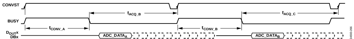
Figure 99. ADC Data Read Can Happen After Conversion and/or During the Following Conversion
