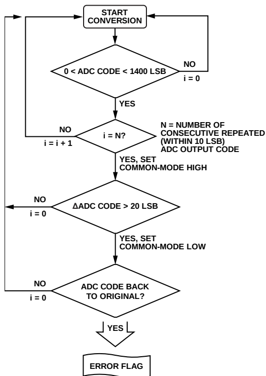
Figure 96. Automatic Analog Input Open Circuit Detect Flowchart
