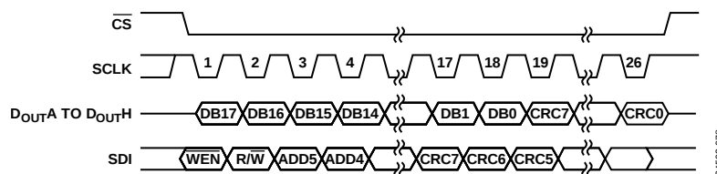
Figure 116. Register Write with CRC On
