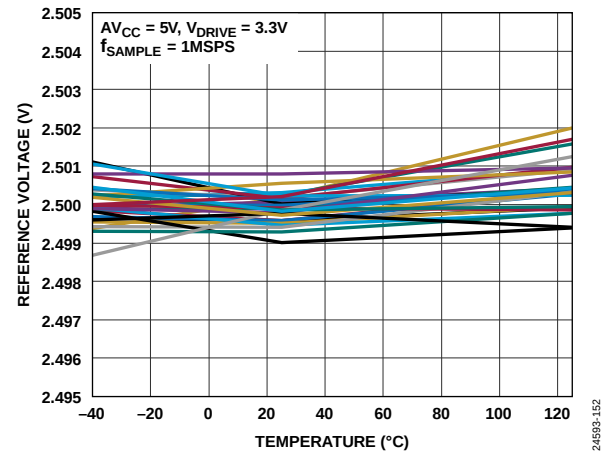
Figure 61. Reference Drift
