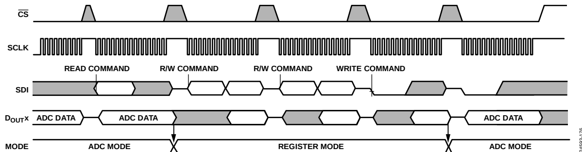
Figure 110. AD7606C-18 Register Mode
