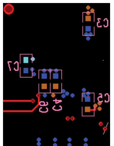
Figure 122. Bottom Layer Decoupling
