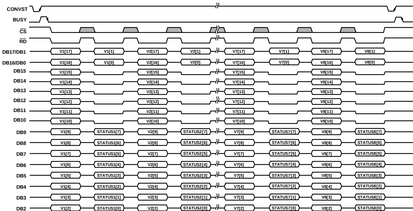
Figure 98. Parallel Interface, ADC Mode with Status Header Enabled
