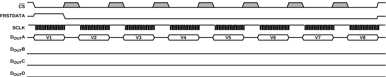
Figure 106. Serial Interface ADC Reading, One DOUTX Line
