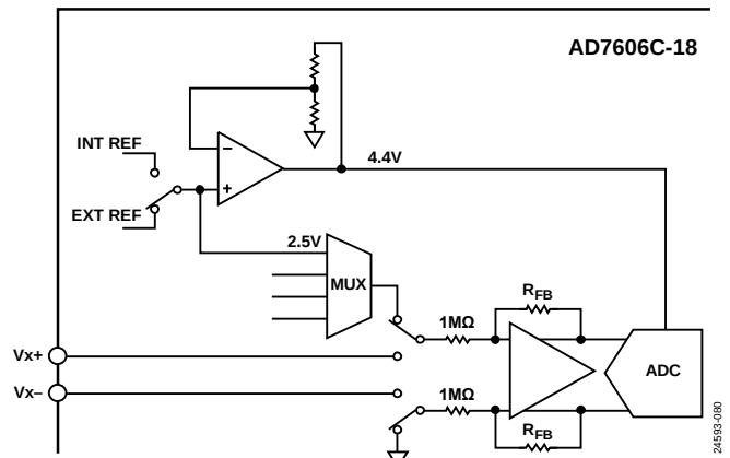
Figure 118. Reference Voltage Signal Path Through the Diagnostic Multiplexer
