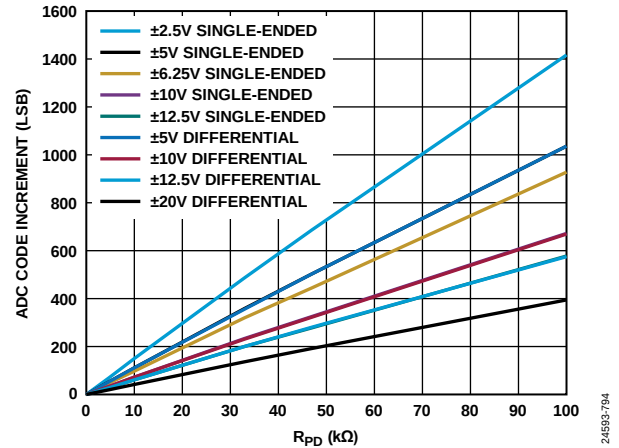
Figure 95. Open Circuit Code Error increment, Dependent of R_{PD}
