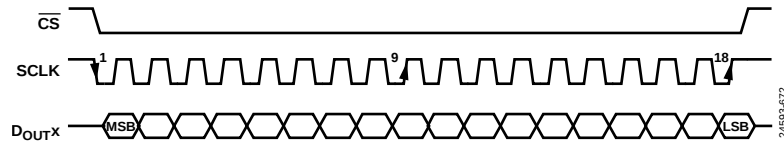
Figure 107. Serial Interface Data Read Back (One Channel)
