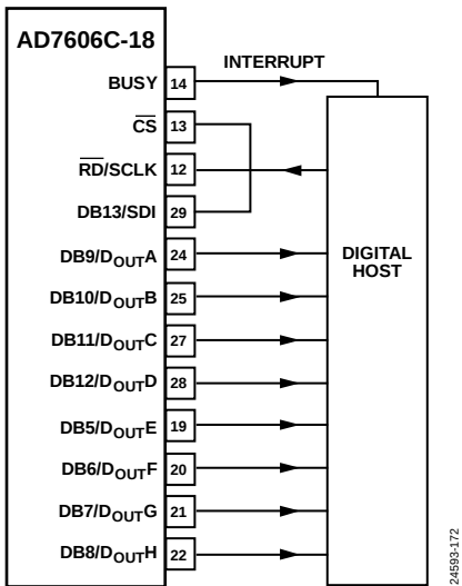
Figure 102. AD7606C-18 Interface Diagram—One AD7606C-18 Using the Serial Interface with Eight DOUTX Lines
