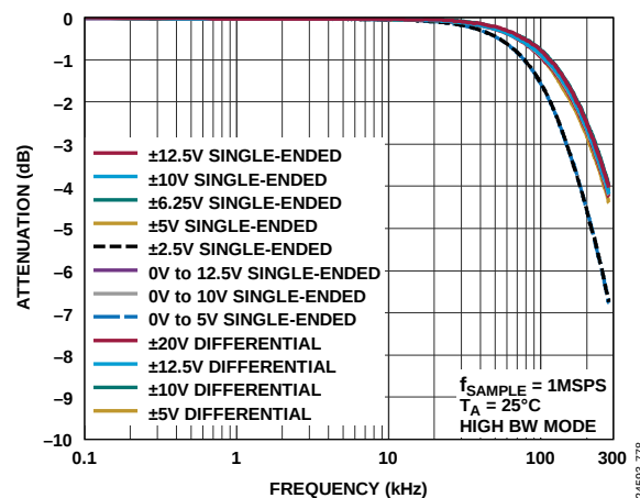
Figure 79. Analog Antialiasing Filter Frequency Response, High Bandwidth Mode
