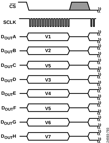
Figure 105. Serial Interface ADC Reading, Eight DOUTX Lines
