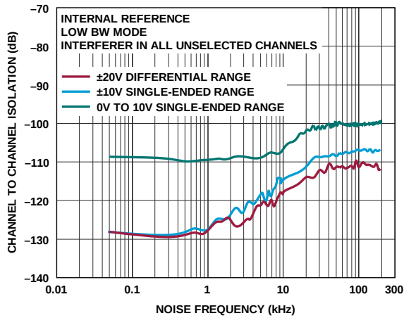
Figure 69. Channel to Channel Isolation vs. Noise Frequency, Low Bandwidth Mode
