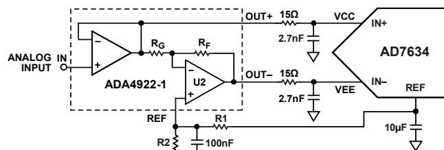
Figure 31. Single-to-Differential Driver Using the ADA4922-1
