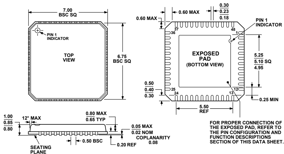
Figure 50. 48-Lead Lead Frame Chip Scale Package [LFCSP_VQ] 7 mm x 7 mm Body, Very Thin Quad (CP-48-1)
