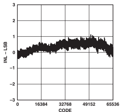
TPC 1. Integral Nonlinearity vs. Code
