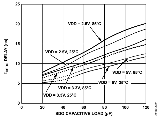
Figure 24. t_{\text{SDO}} Delay vs. Capacitance Load and Supply
