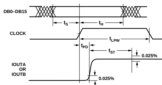
Timing Diagram
