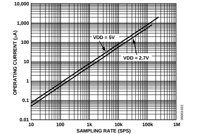
Figure 22. Operating Current vs. Sampling Rate
