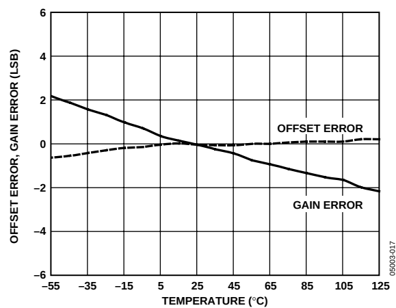
Figure 17. Offset and Gain Error vs. Temperature
