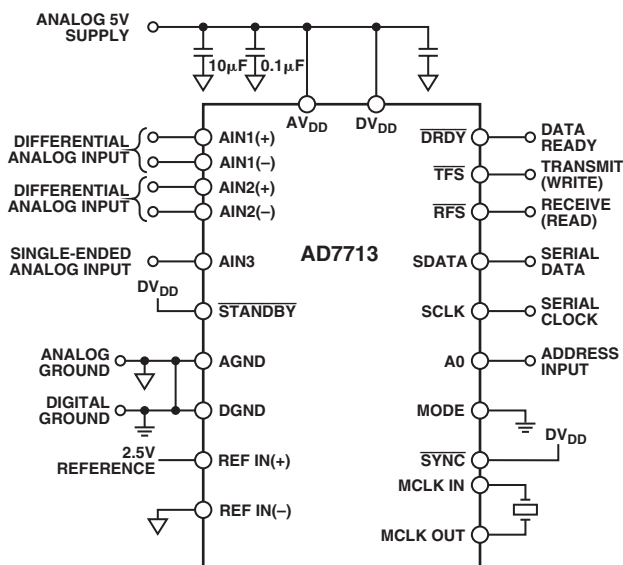
Figure 3. Basic Connection Diagram
