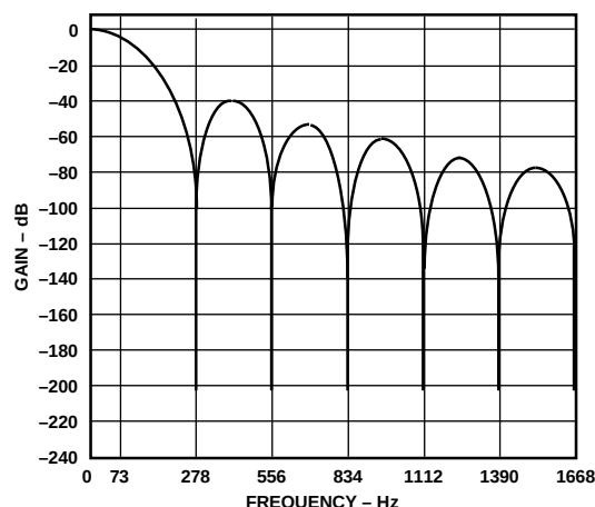
Figure 6. Frequency Response of AD7716 Filter
