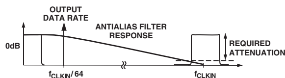
Figure 10b. Frequency Response of Antialias Filter
