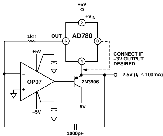
Figure 25. -2.5 V High Load Current Reference
