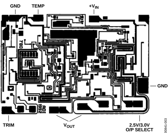
Figure 3. Die Layout
