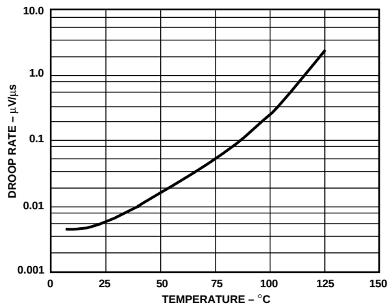
Droop Rate vs. Temperature, V_{IN} = 0 V
