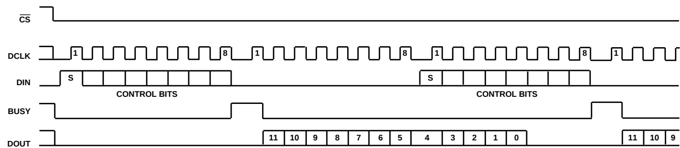
Figure 26. Conversion Timing, 16 DCLKS per Cycle, 8-Bit Bus Interface. No DCLK delay required with dedicated serial port.
