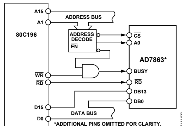
Figure 23. AD7863–80C196 Interface
